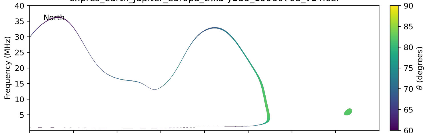
expres_earth_jupiter_europa_txka-y235_19960708_v14.cdf
