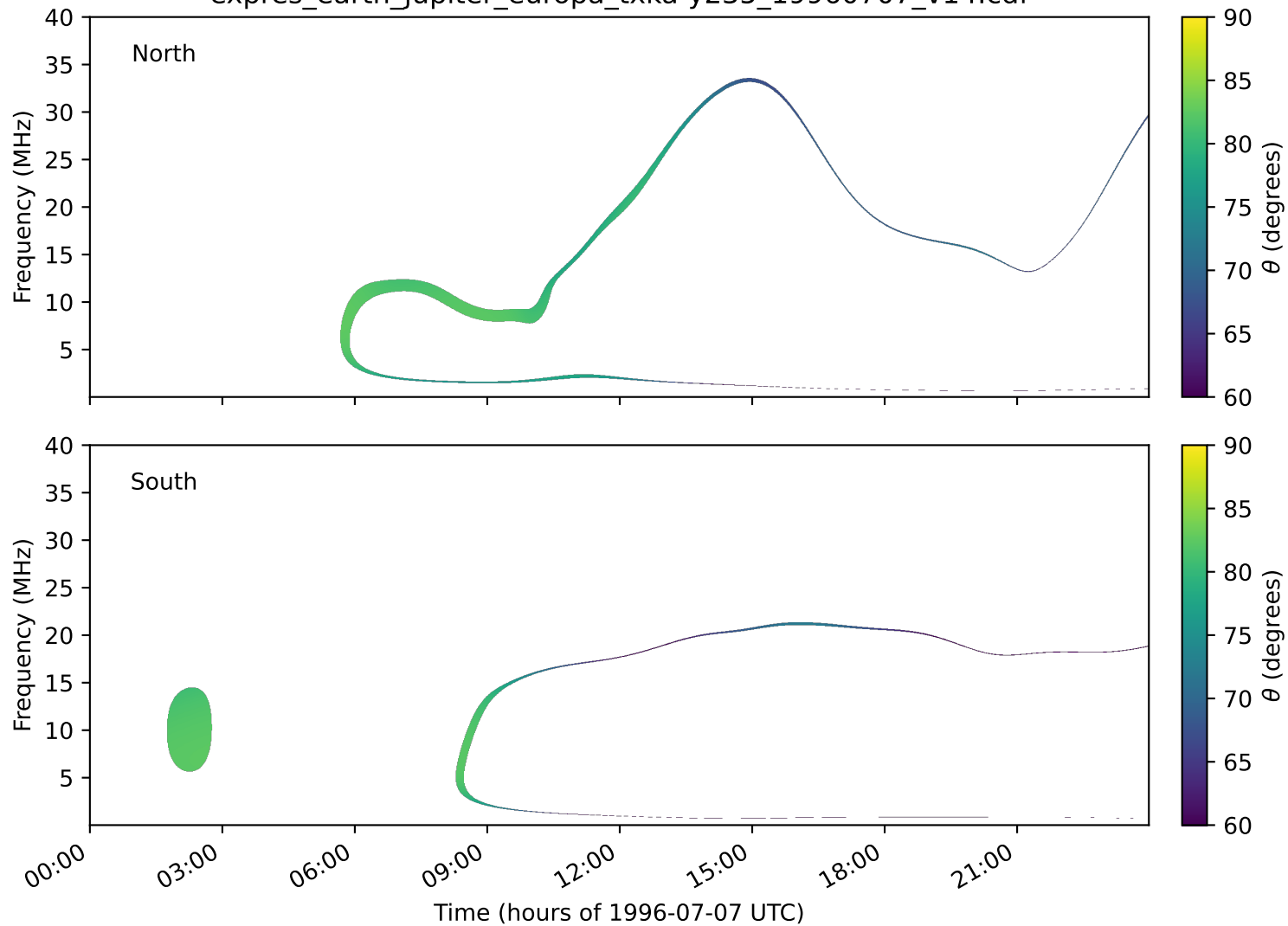
expres_earth_jupiter_europa_txka-y235_19960707_v14.cdf
