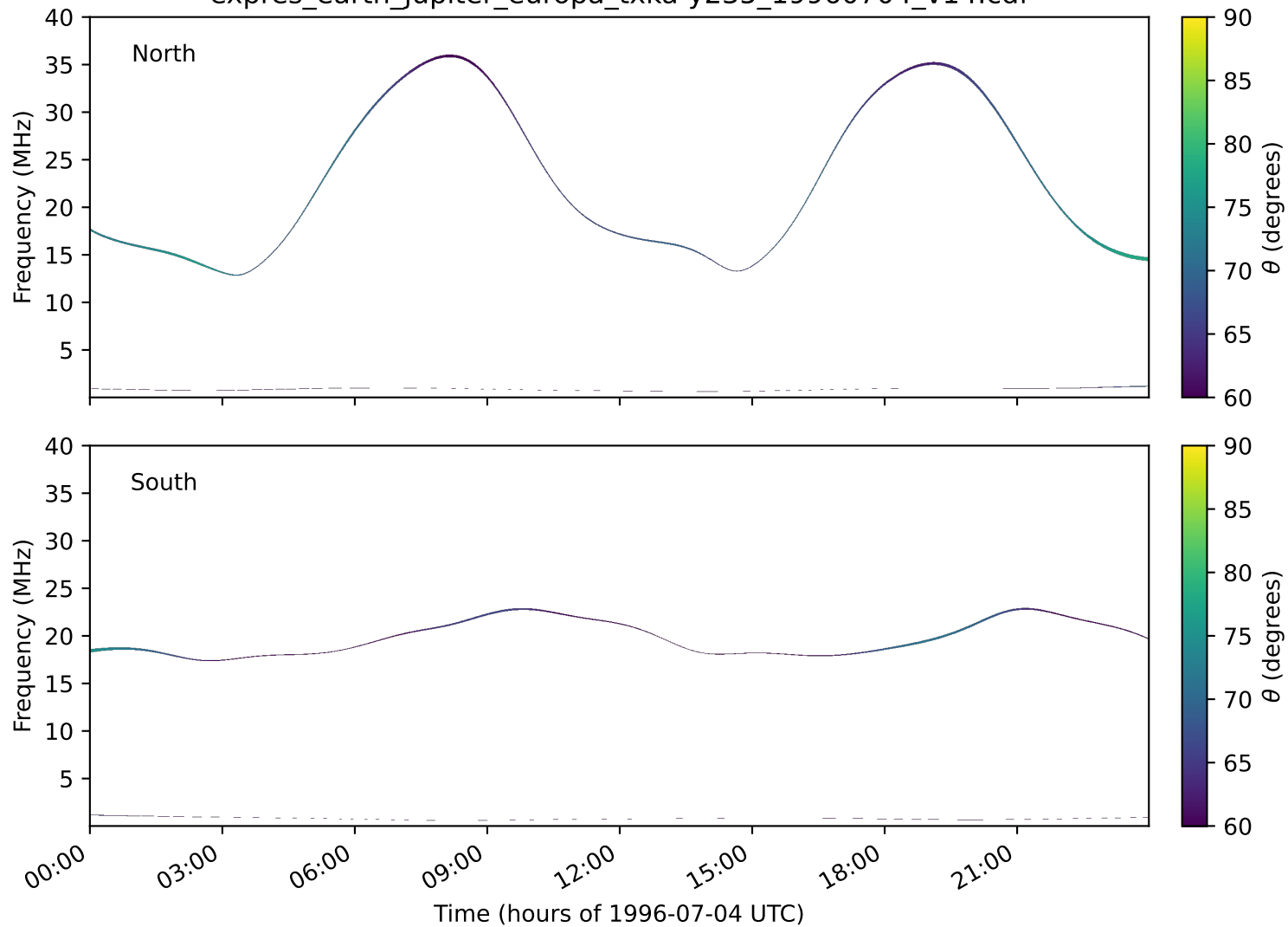
expres_earth_jupiter_europa_txka-y235_19960704_v14.cdf
