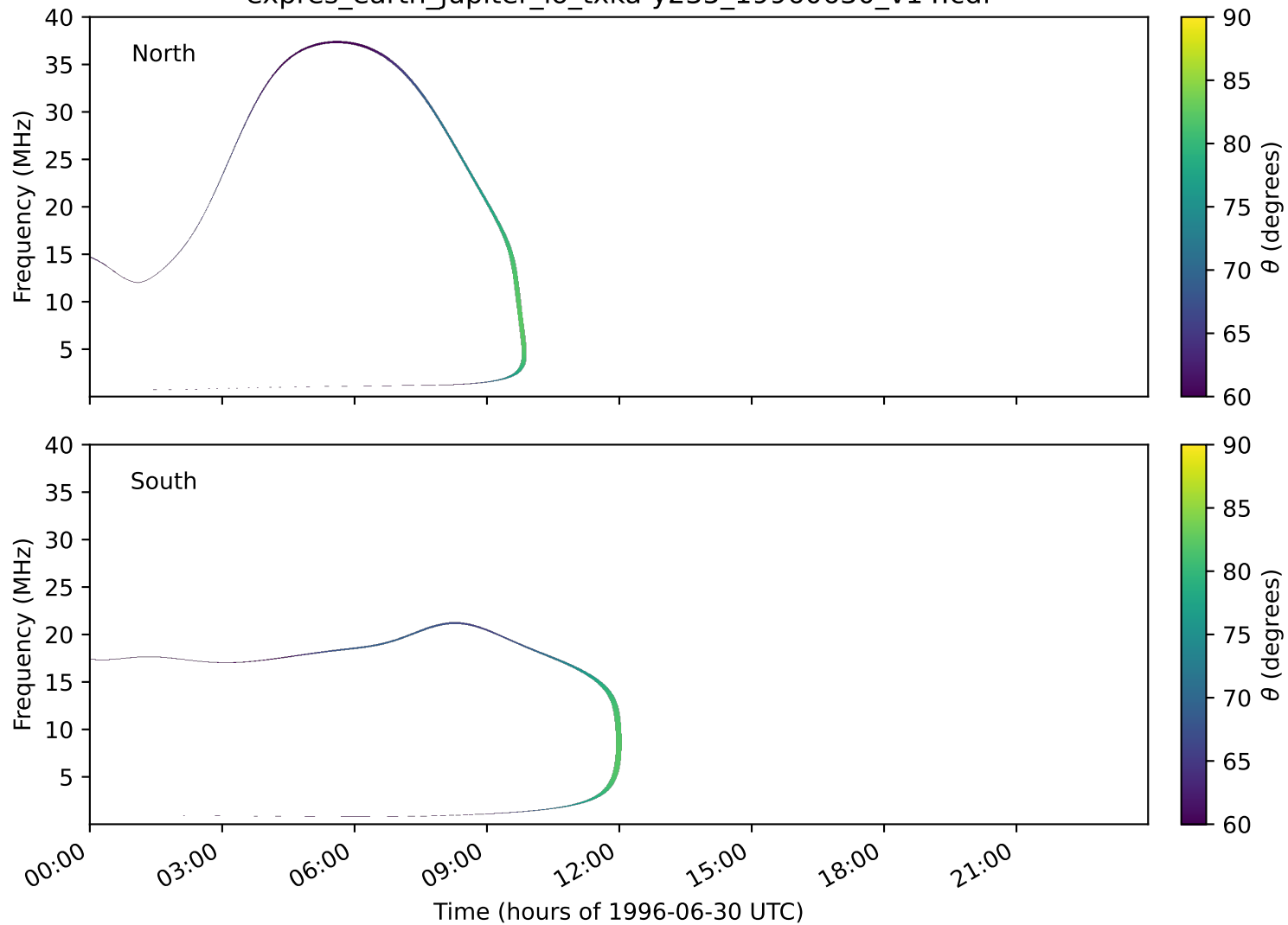
expres_earth_jupiter_io_txka-y235_19960630_v14.cdf
