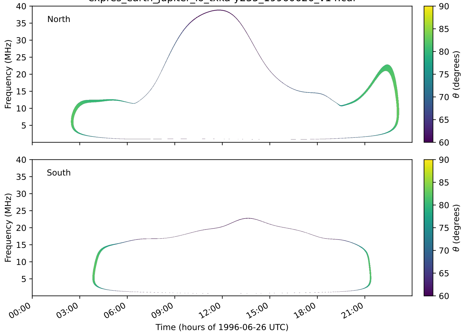
expres_earth_jupiter_io_txka-y235_19960626_v14.cdf
