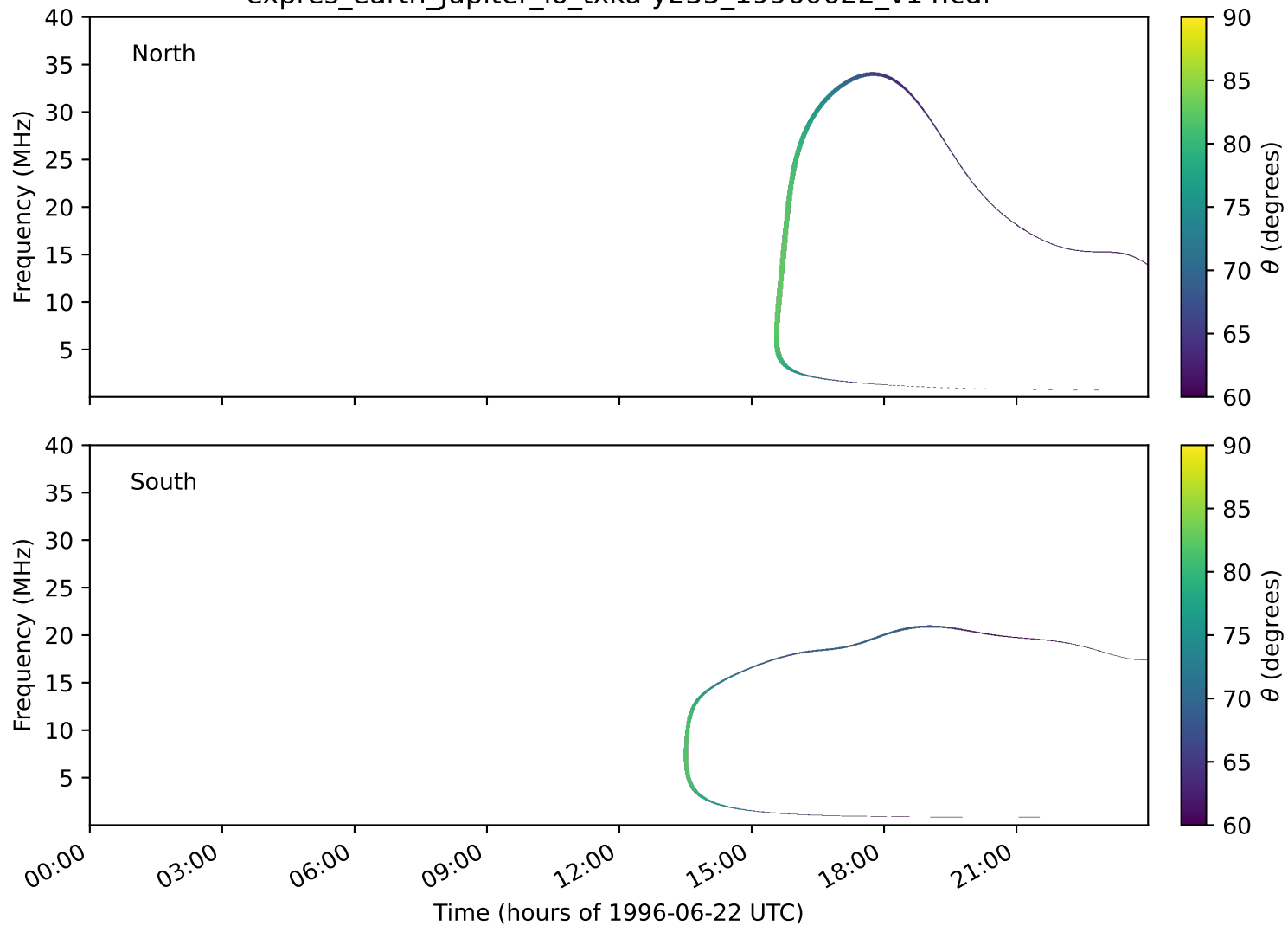
expres_earth_jupiter_io_txka-y235_19960622_v14.cdf
