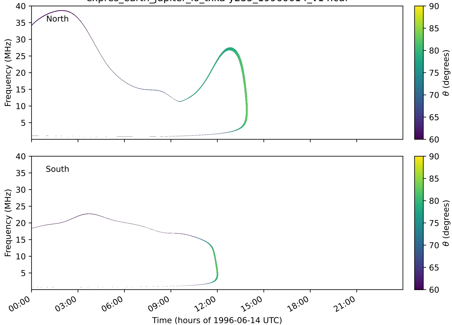
expres_earth_jupiter_io_txka-y235_19960614_v14.cdf
