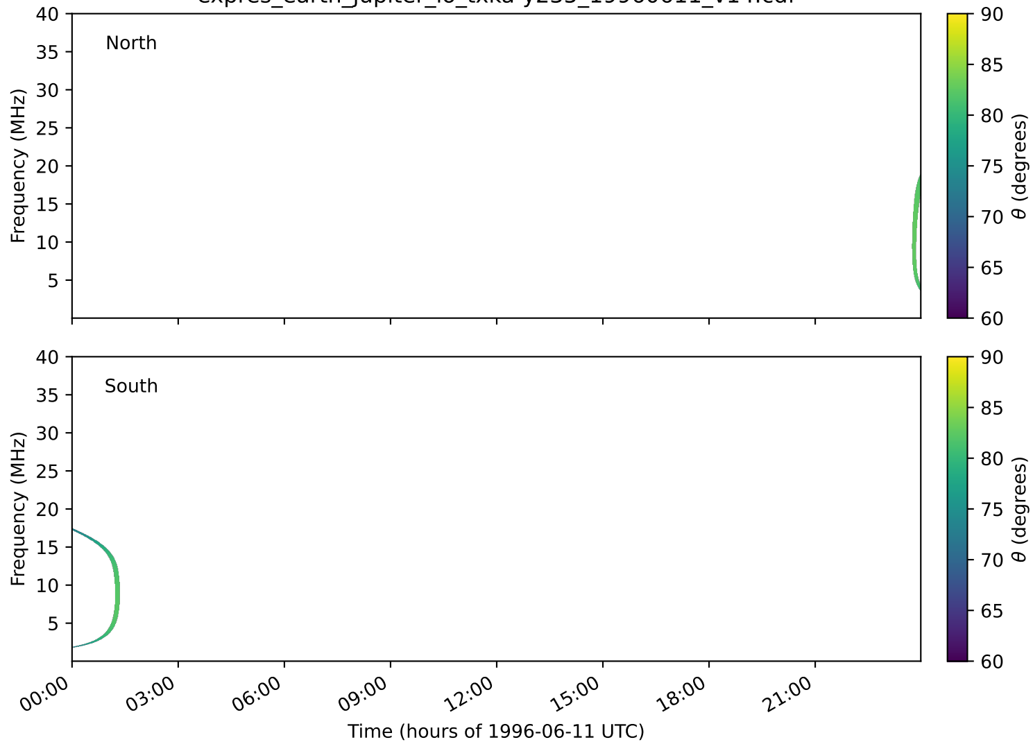
expres_earth_jupiter_io_txka-y235_19960611_v14.cdf
