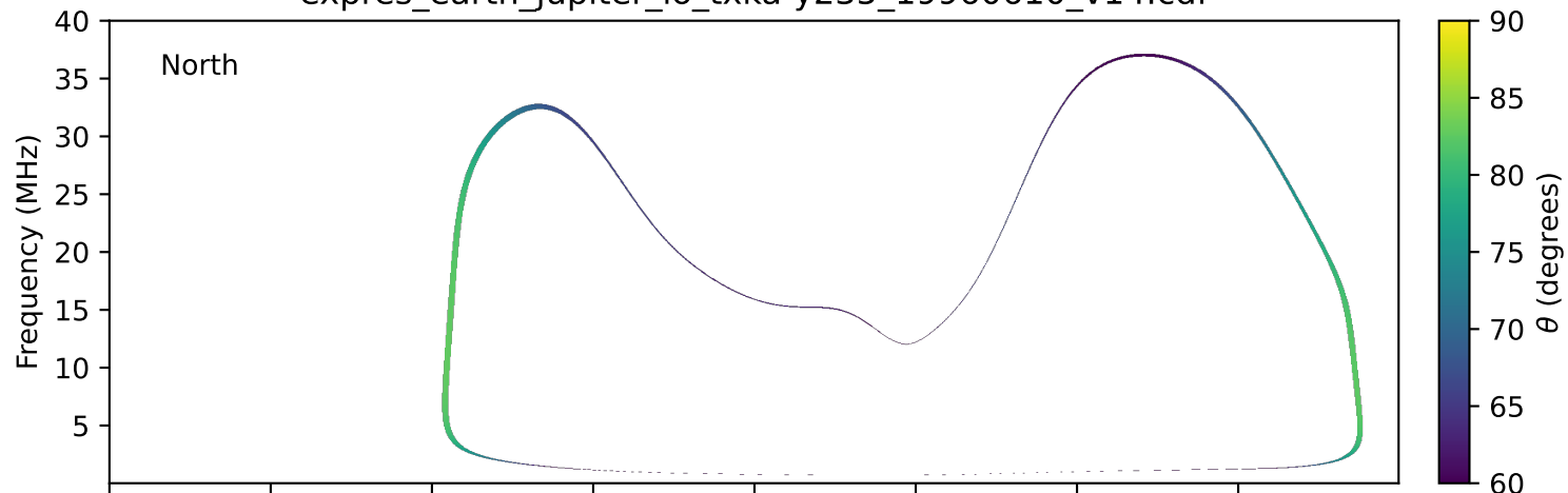
expres_earth_jupiter_io_txka-y235_19960610_v14.cdf
