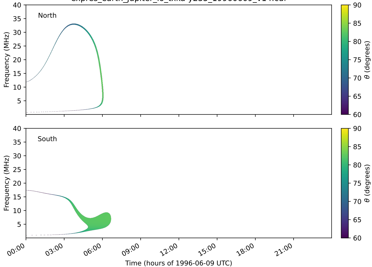
expres_earth_jupiter_io_txka-y235_19960609_v14.cdf
