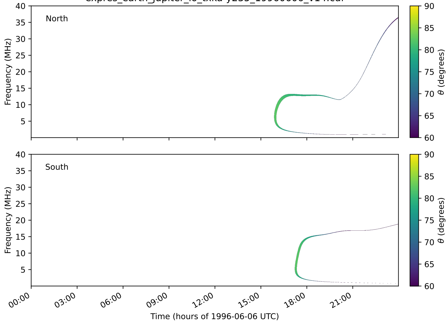
expres_earth_jupiter_io_txka-y235_19960606_v14.cdf
