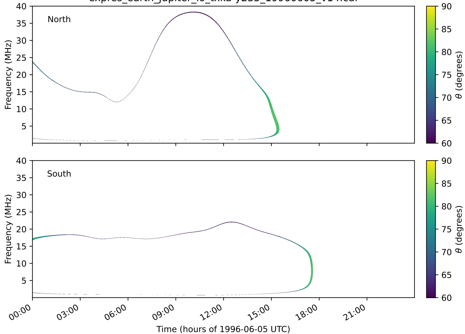
expres_earth_jupiter_io_txka-y235_19960605_v14.cdf
