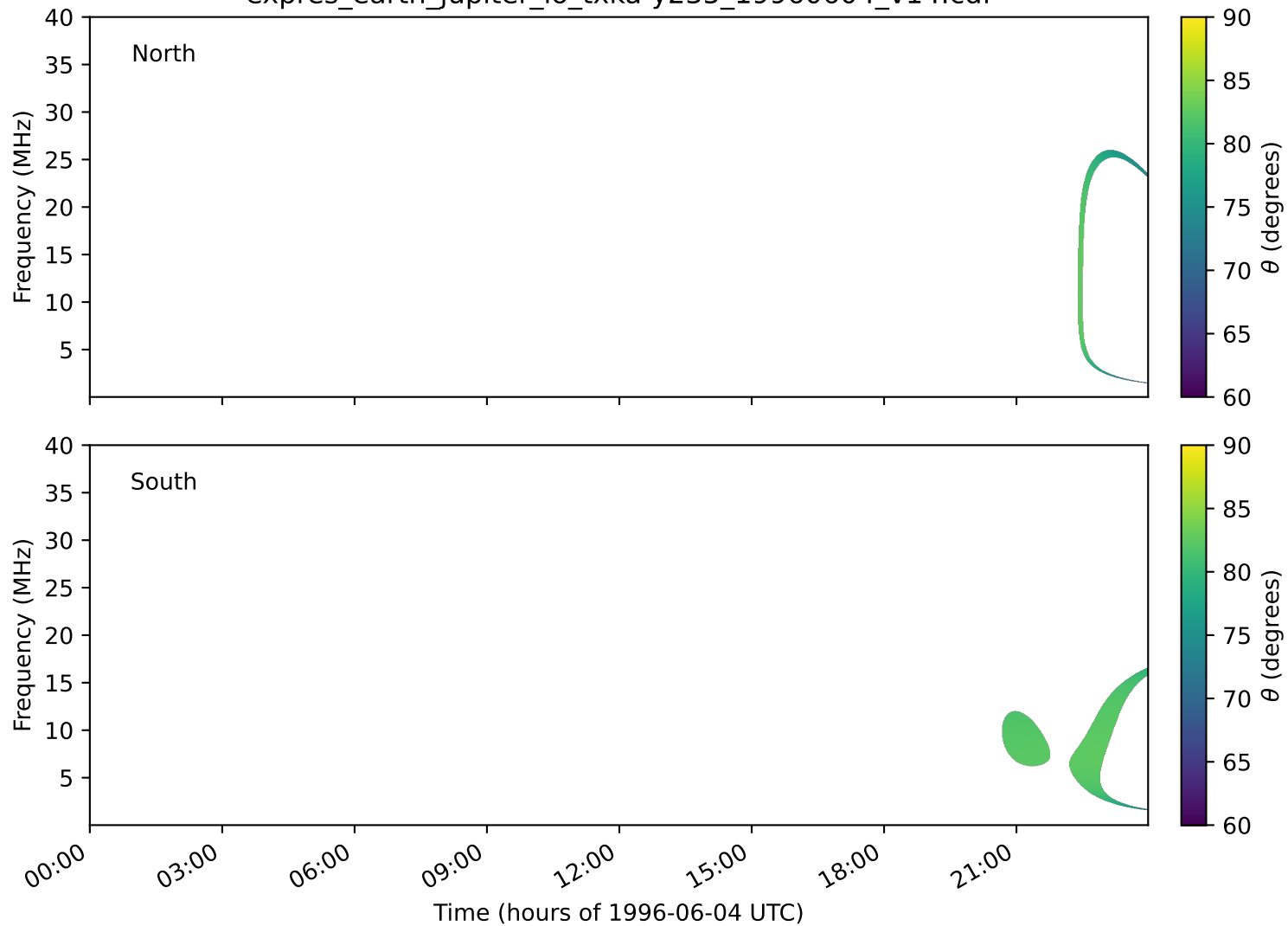
expres_earth_jupiter_io_txka-y235_19960604_v14.cdf
