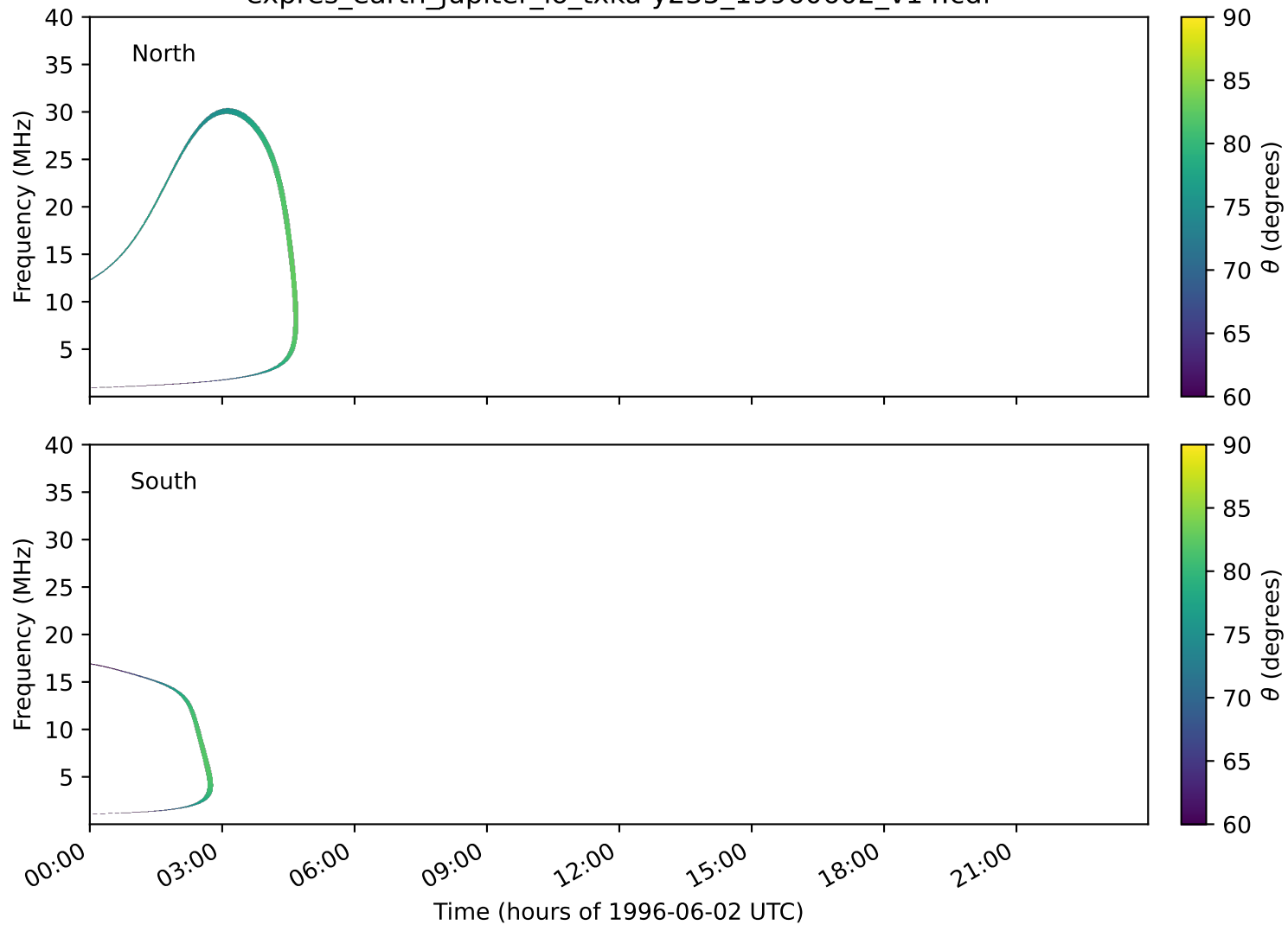
expres_earth_jupiter_io_txka-y235_19960602_v14.cdf
