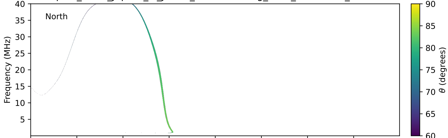
expres_earth_jupiter_io_jrm33_lossc-wid1deg_3kev_19960623_v11.cdf
