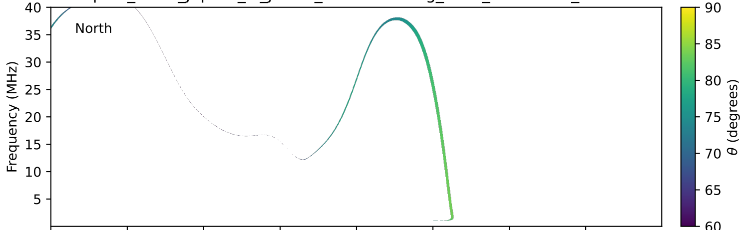
expres_earth_jupiter_io_jrm33_lossc-wid1deg_3kev_19960621_v11.cdf
