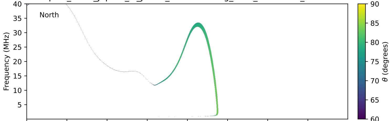
expres_earth_jupiter_io_jrm33_lossc-wid1deg_3kev_19960614_v11.cdf
