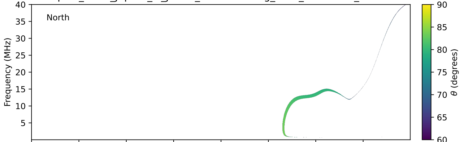
expres_earth_jupiter_io_jrm33_lossc-wid1deg_3kev_19960606_v11.cdf
