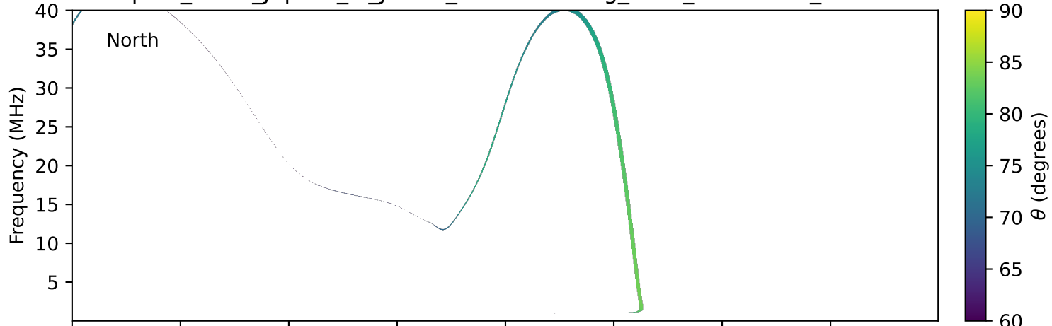
expres_earth_jupiter_io_jrm09_lossc-wid1deg_3kev_19960621_v11.cdf
