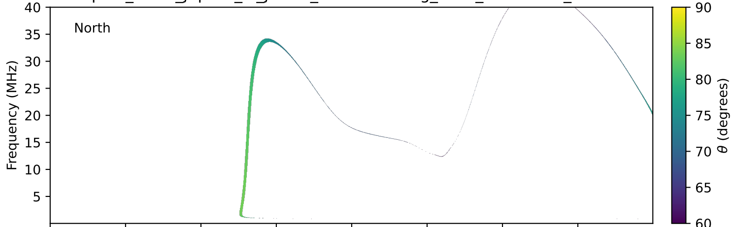
expres_earth_jupiter_io_jrm09_lossc-wid1deg_3kev_19960617_v11.cdf
