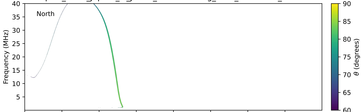
expres_earth_jupiter_io_jrm09_lossc-wid1deg_3kev_19960616_v11.cdf
