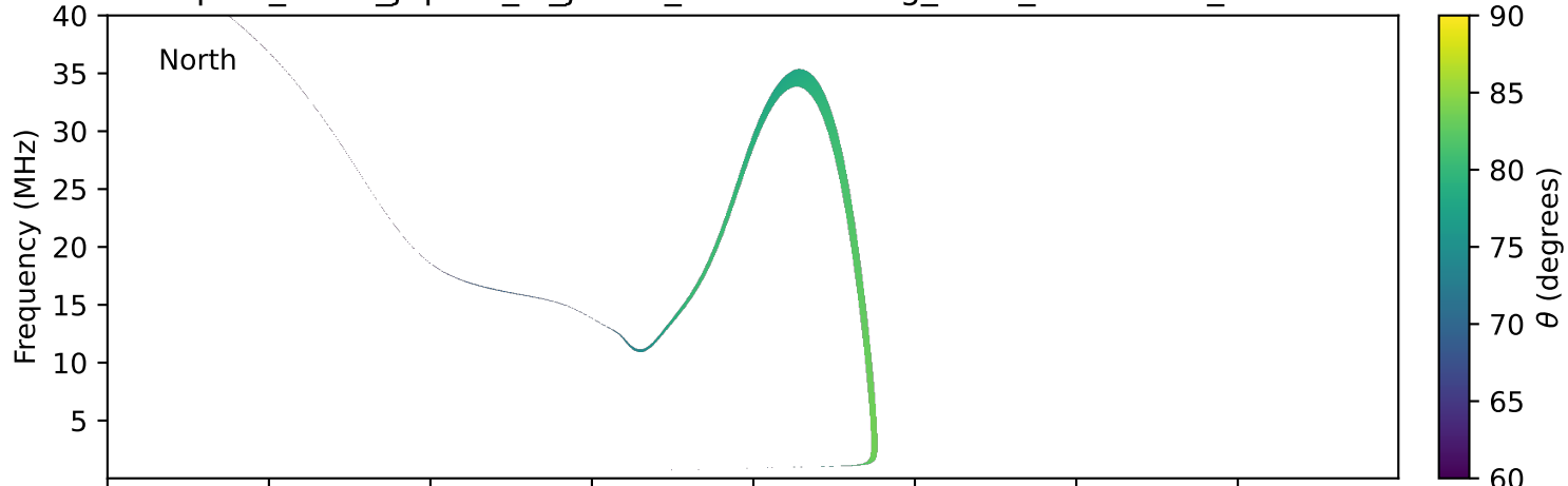
expres_earth_jupiter_io_jrm09_lossc-wid1deg_3kev_19960614_v11.cdf
