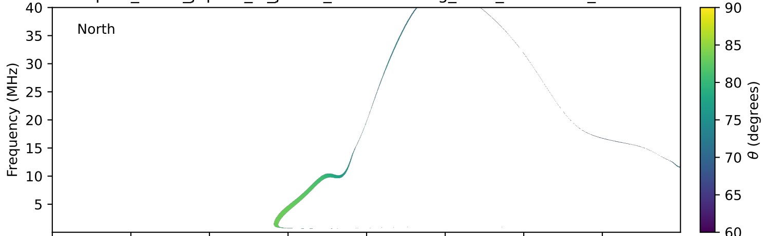
expres_earth_jupiter_io_jrm09_lossc-wid1deg_3kev_19960601_v11.cdf
