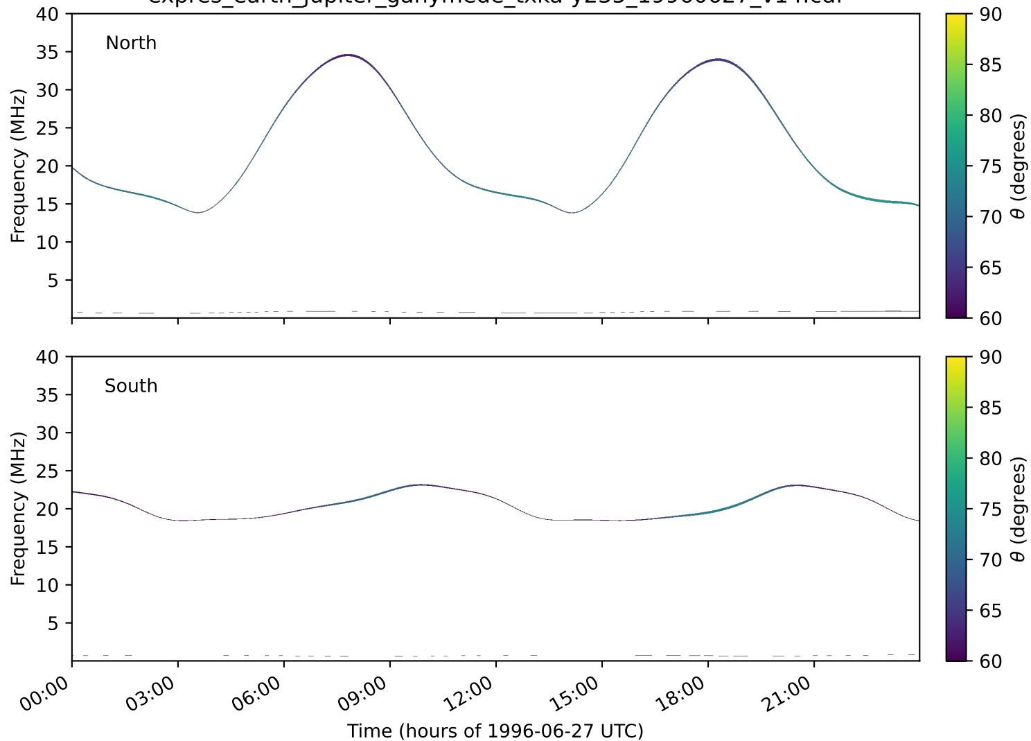
expres_earth_jupiter_ganymede_txka-y235_19960627_v14.cdf
