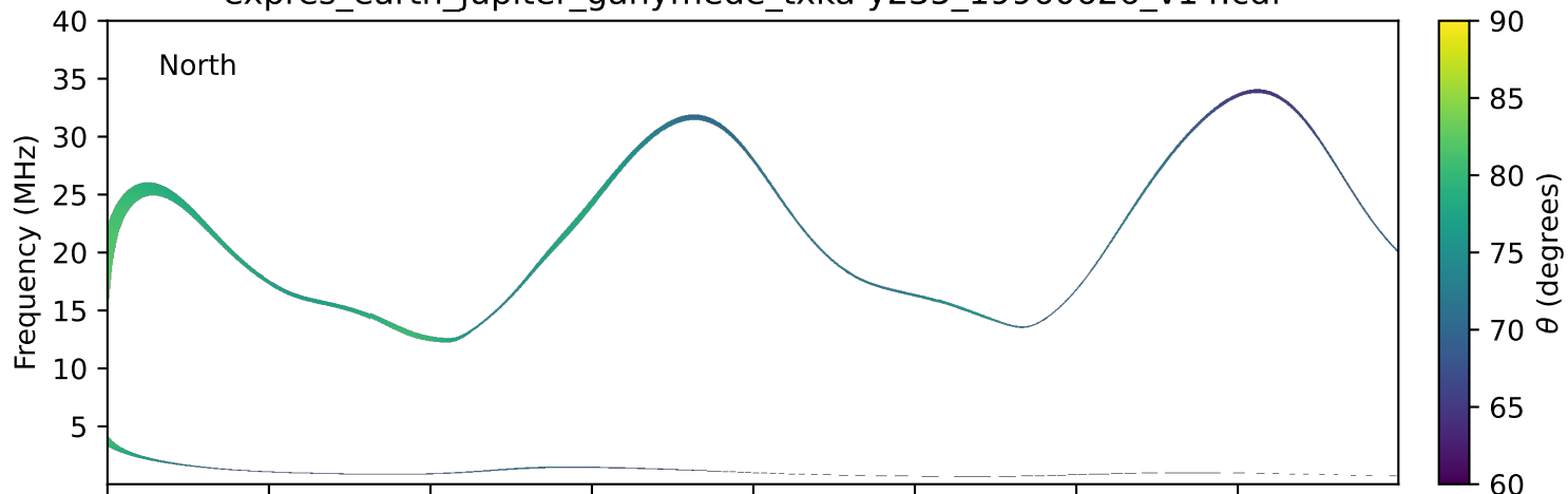
expres_earth_jupiter_ganymede_txka-y235_19960626_v14.cdf
