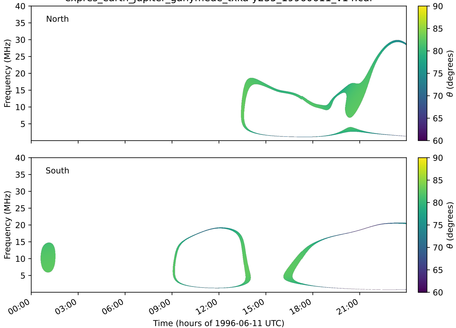
expres_earth_jupiter_ganymede_txka-y235_19960611_v14.cdf
