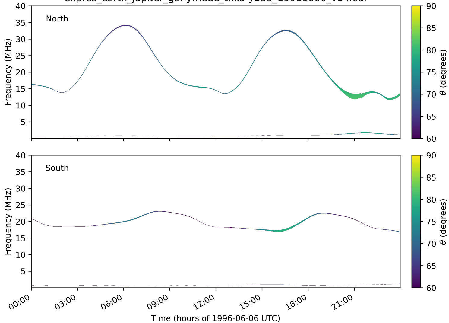
expres_earth_jupiter_ganymede_txka-y235_19960606_v14.cdf
