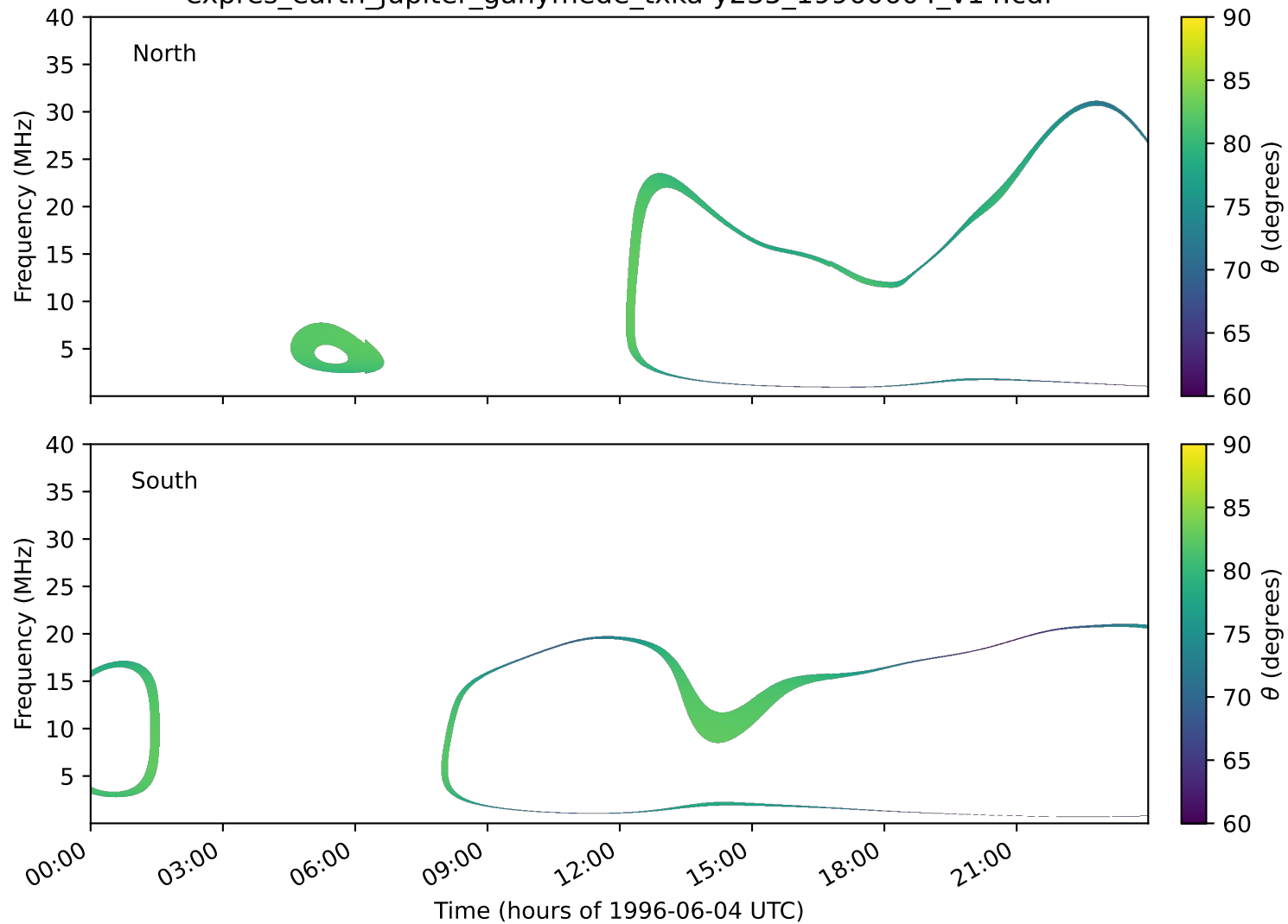
expres_earth_jupiter_ganymede_txka-y235_19960604_v14.cdf
