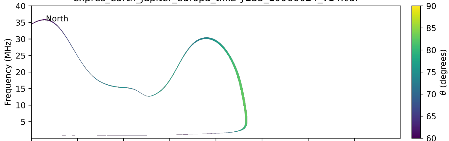
expres_earth_jupiter_europa_txka-y235_19960624_v14.cdf
