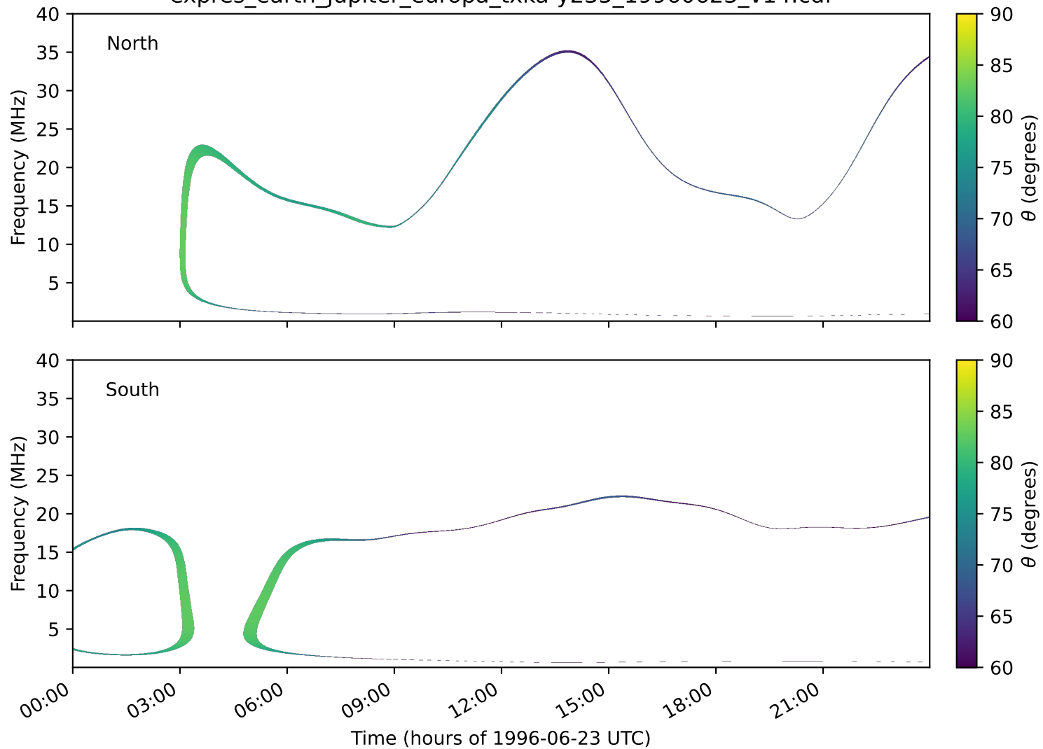
expres_earth_jupiter_europa_txka-y235_19960623_v14.cdf
