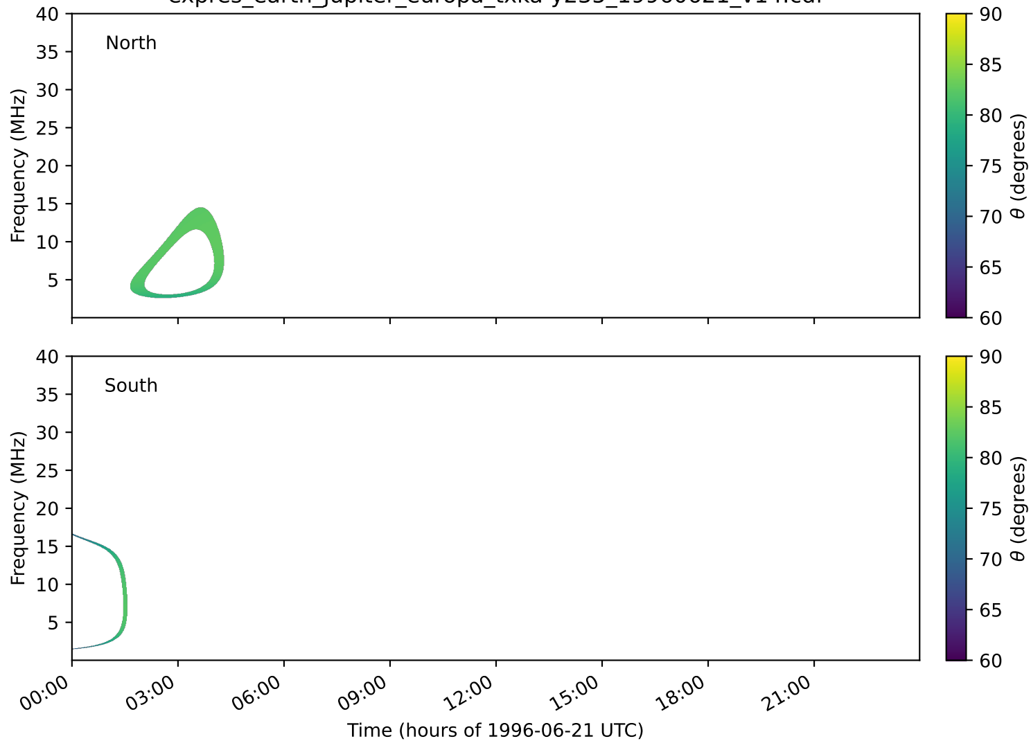
expres_earth_jupiter_europa_txka-y235_19960621_v14.cdf
