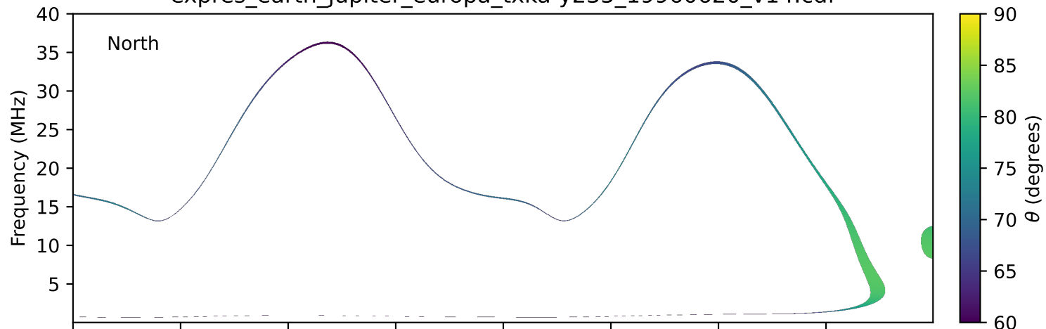
expres_earth_jupiter_europa_txka-y235_19960620_v14.cdf
