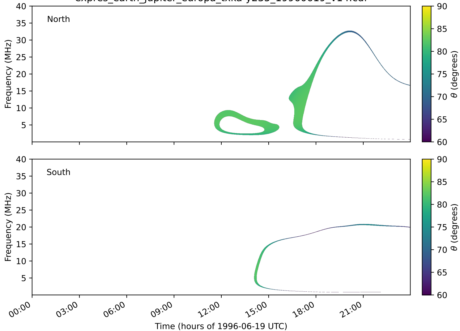
expres_earth_jupiter_europa_txka-y235_19960619_v14.cdf
