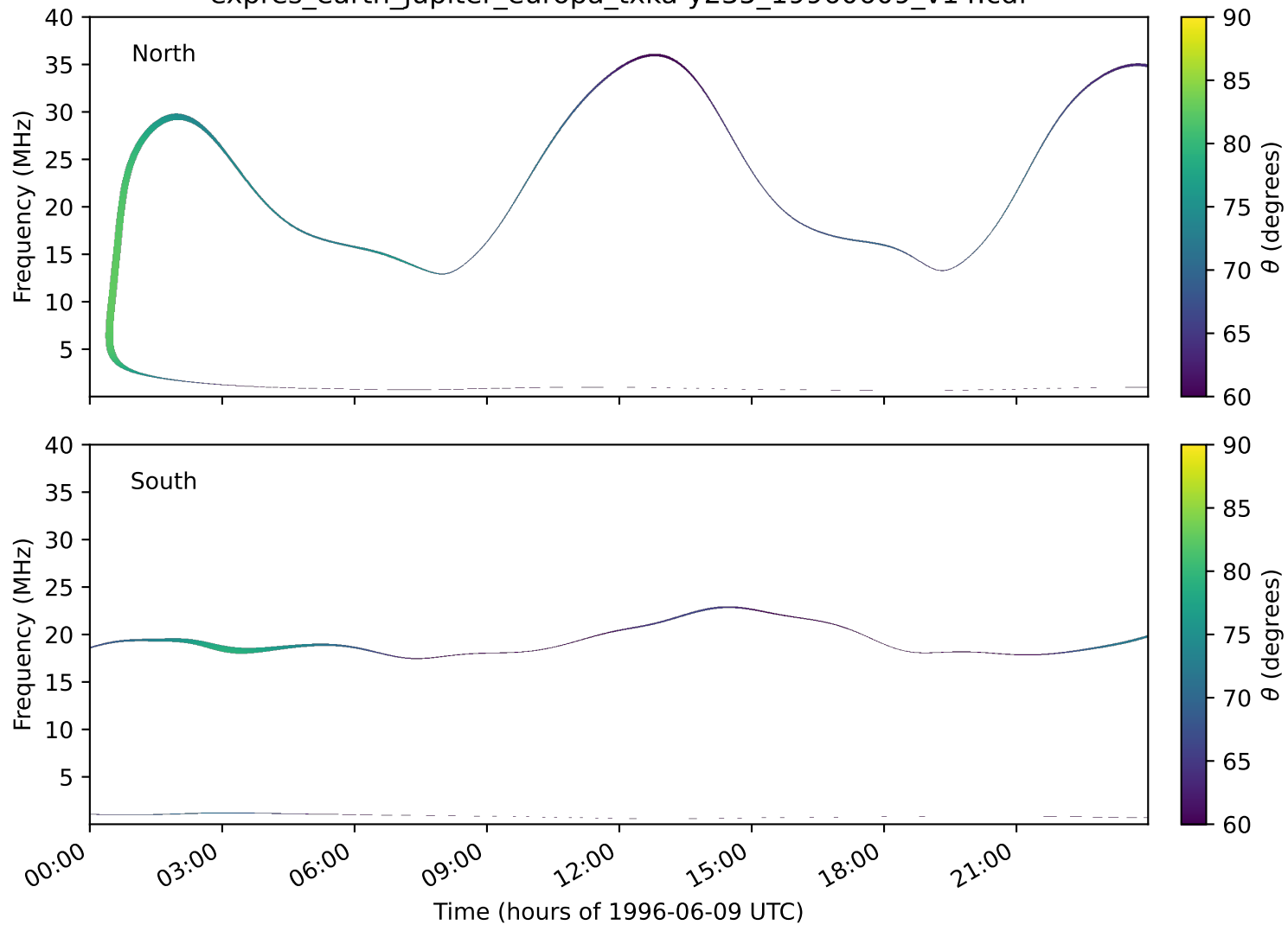
expres_earth_jupiter_europa_txka-y235_19960609_v14.cdf
