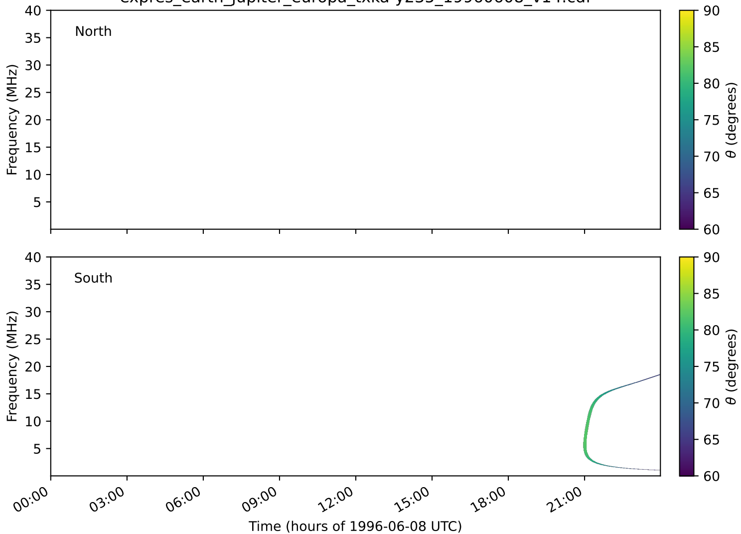
expres_earth_jupiter_europa_txka-y235_19960608_v14.cdf
