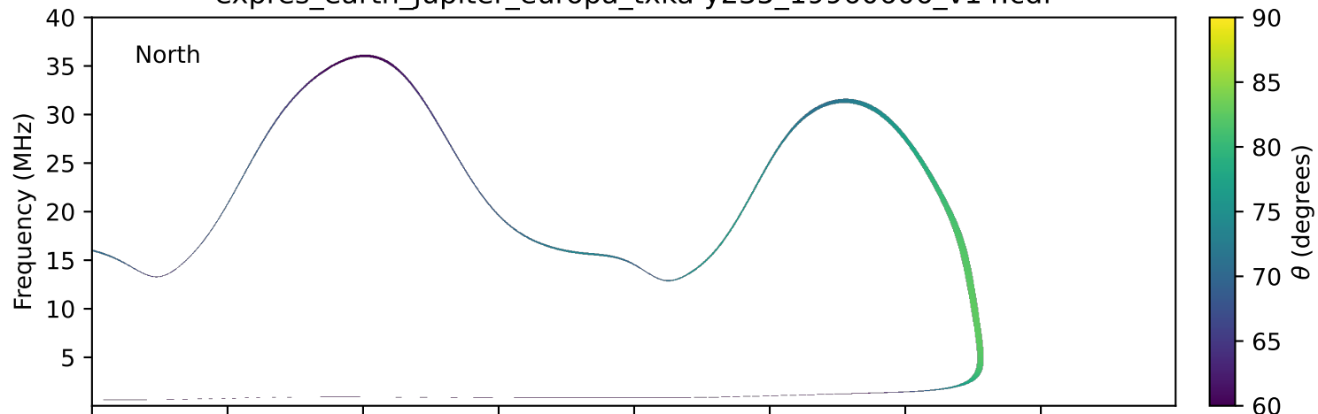
expres_earth_jupiter_europa_txka-y235_19960606_v14.cdf
