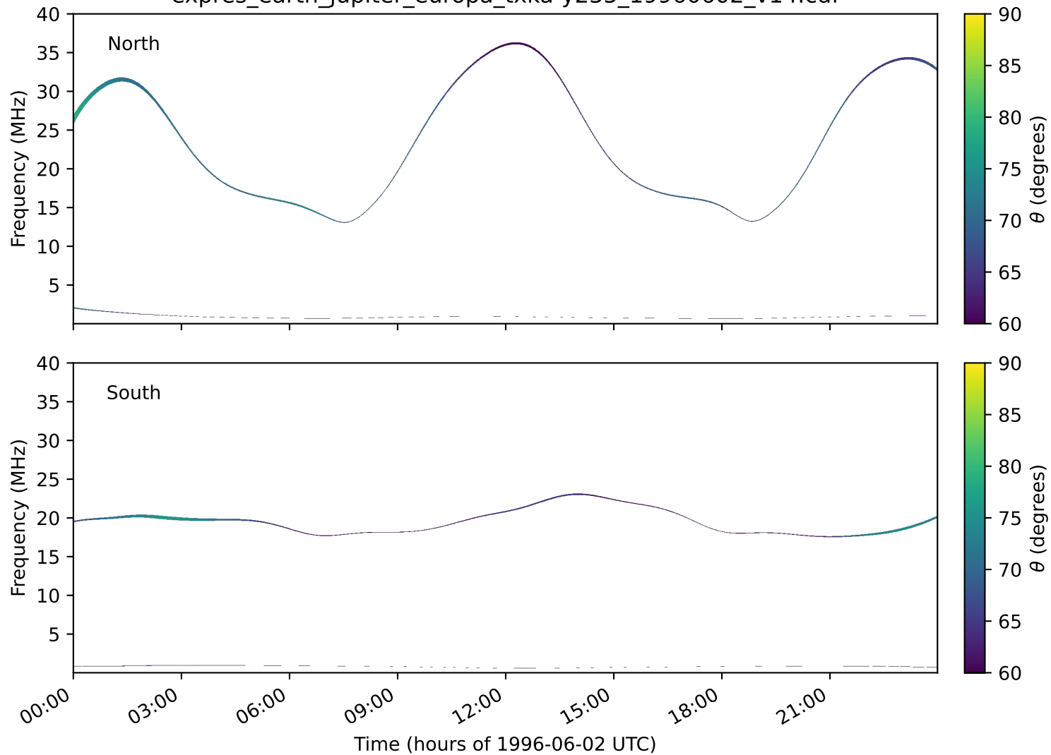
expres_earth_jupiter_europa_txka-y235_19960602_v14.cdf
