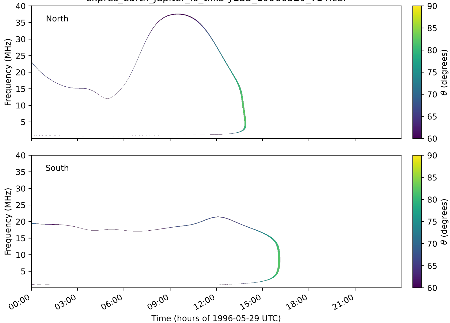
expres_earth_jupiter_io_txka-y235_19960529_v14.cdf
