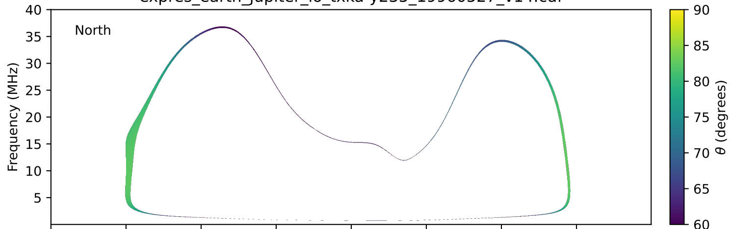
expres_earth_jupiter_io_txka-y235_19960527_v14.cdf
