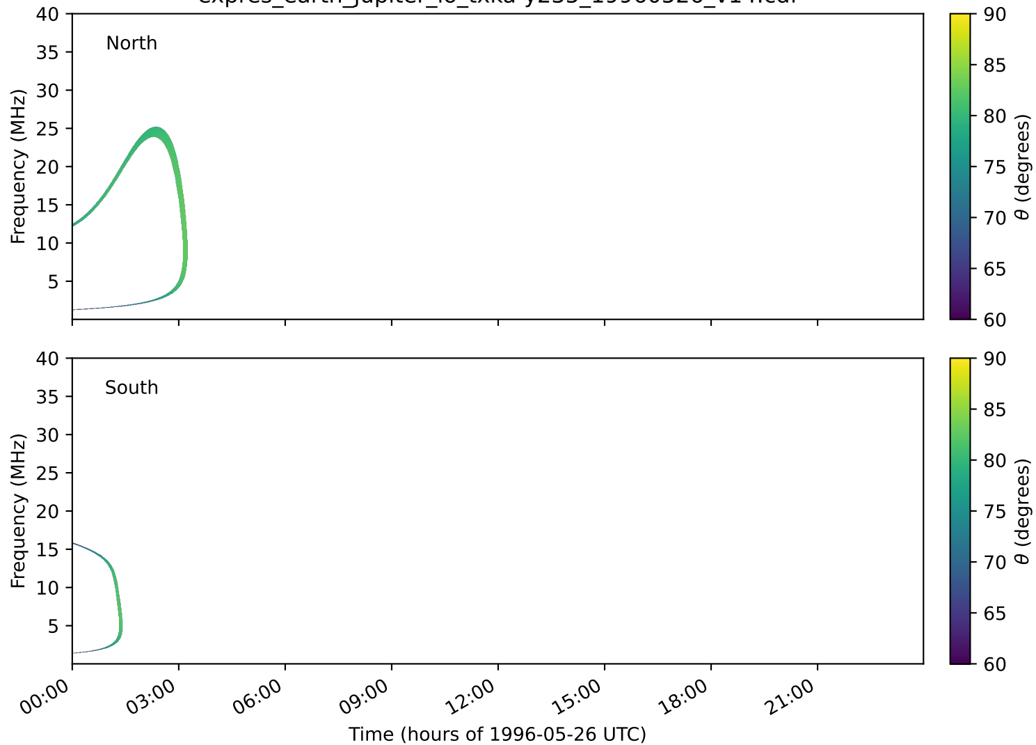
expres_earth_jupiter_io_txka-y235_19960526_v14.cdf
