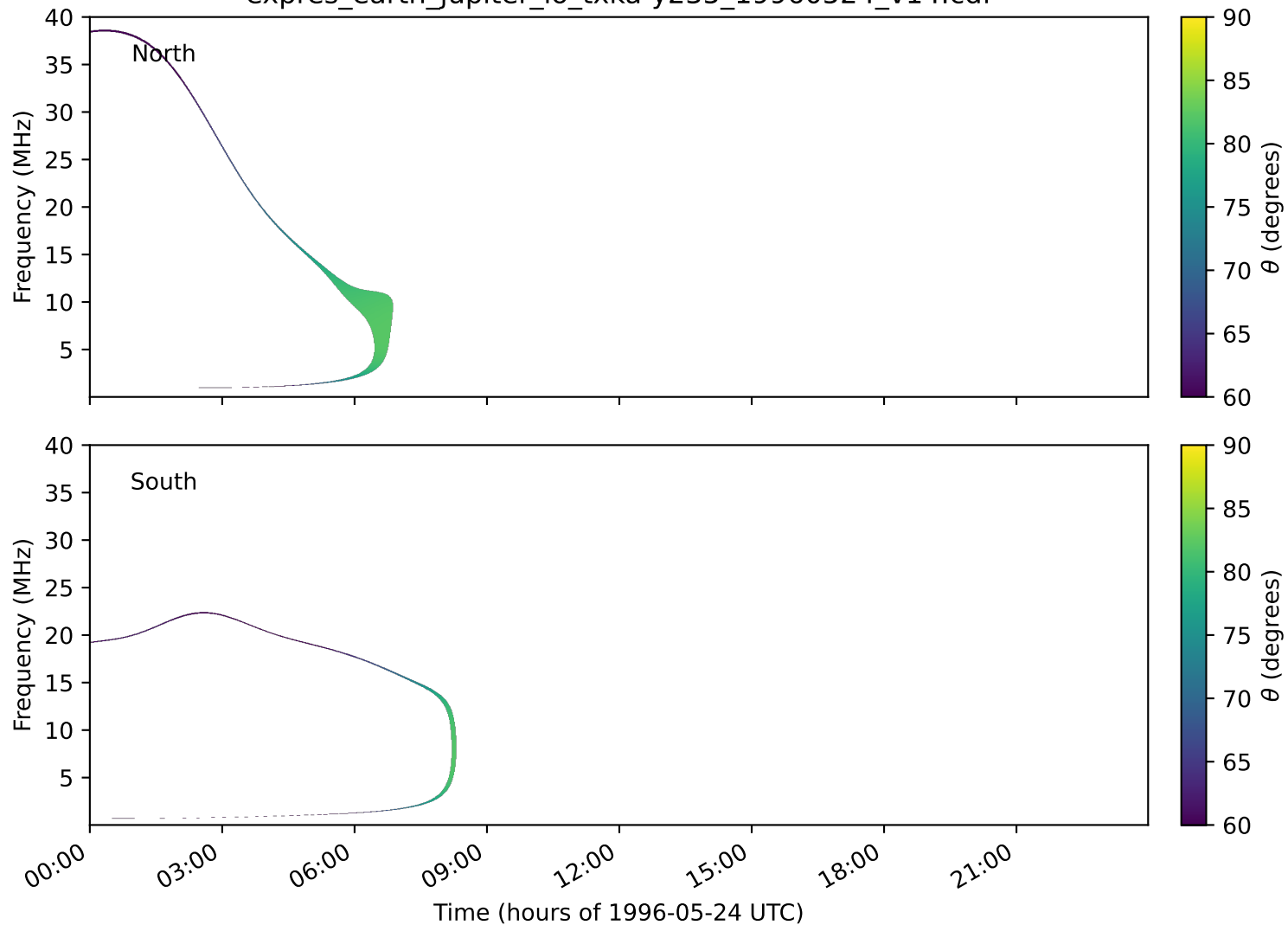
expres_earth_jupiter_io_txka-y235_19960524_v14.cdf
