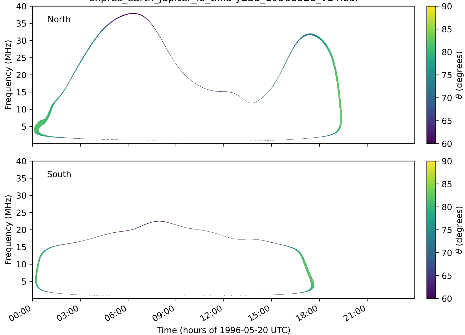
expres_earth_jupiter_io_txka-y235_19960520_v14.cdf
