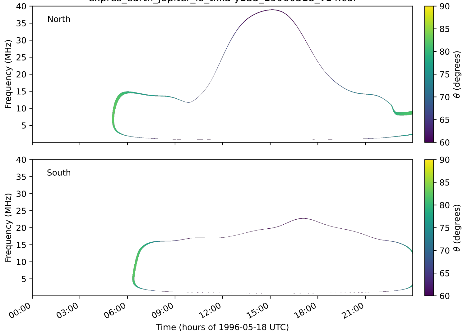
expres_earth_jupiter_io_txka-y235_19960518_v14.cdf
