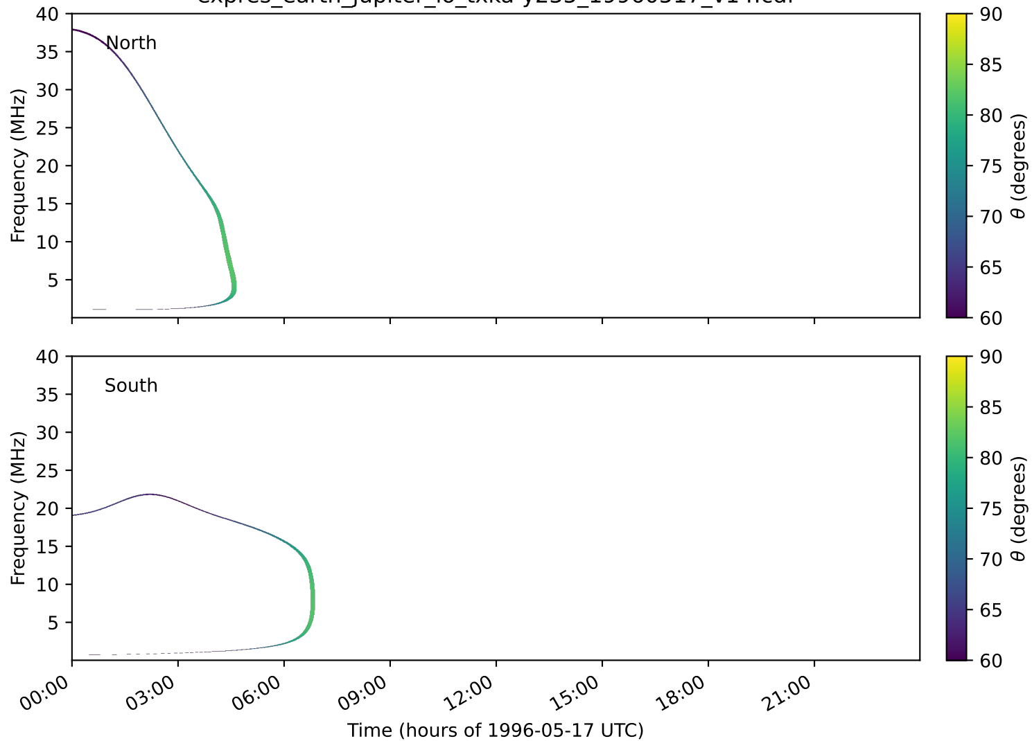
expres_earth_jupiter_io_txka-y235_19960517_v14.cdf
