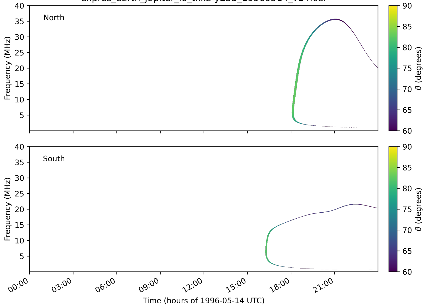
expres_earth_jupiter_io_txka-y235_19960514_v14.cdf
