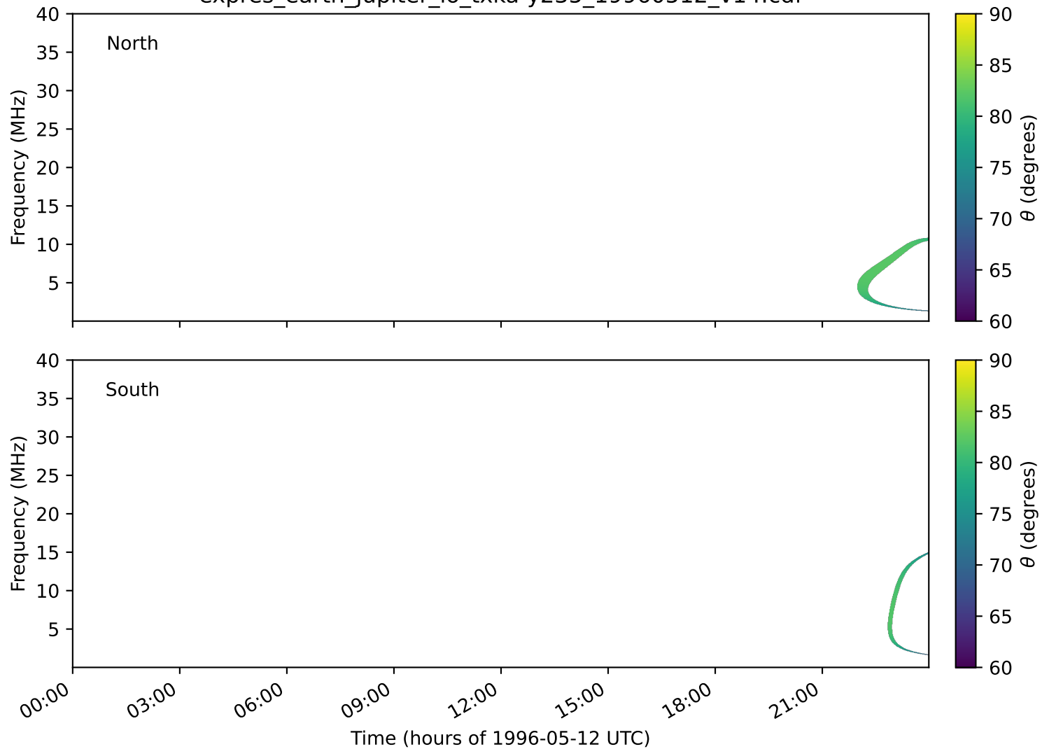
expres_earth_jupiter_io_txka-y235_19960512_v14.cdf
