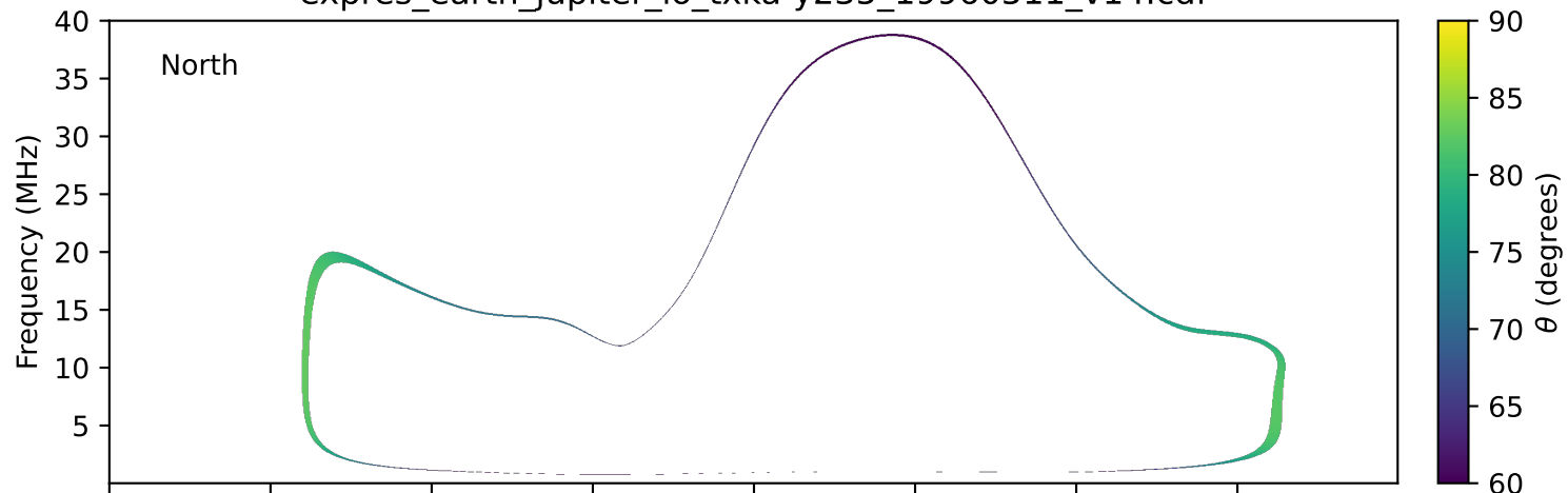
expres_earth_jupiter_io_txka-y235_19960511_v14.cdf
