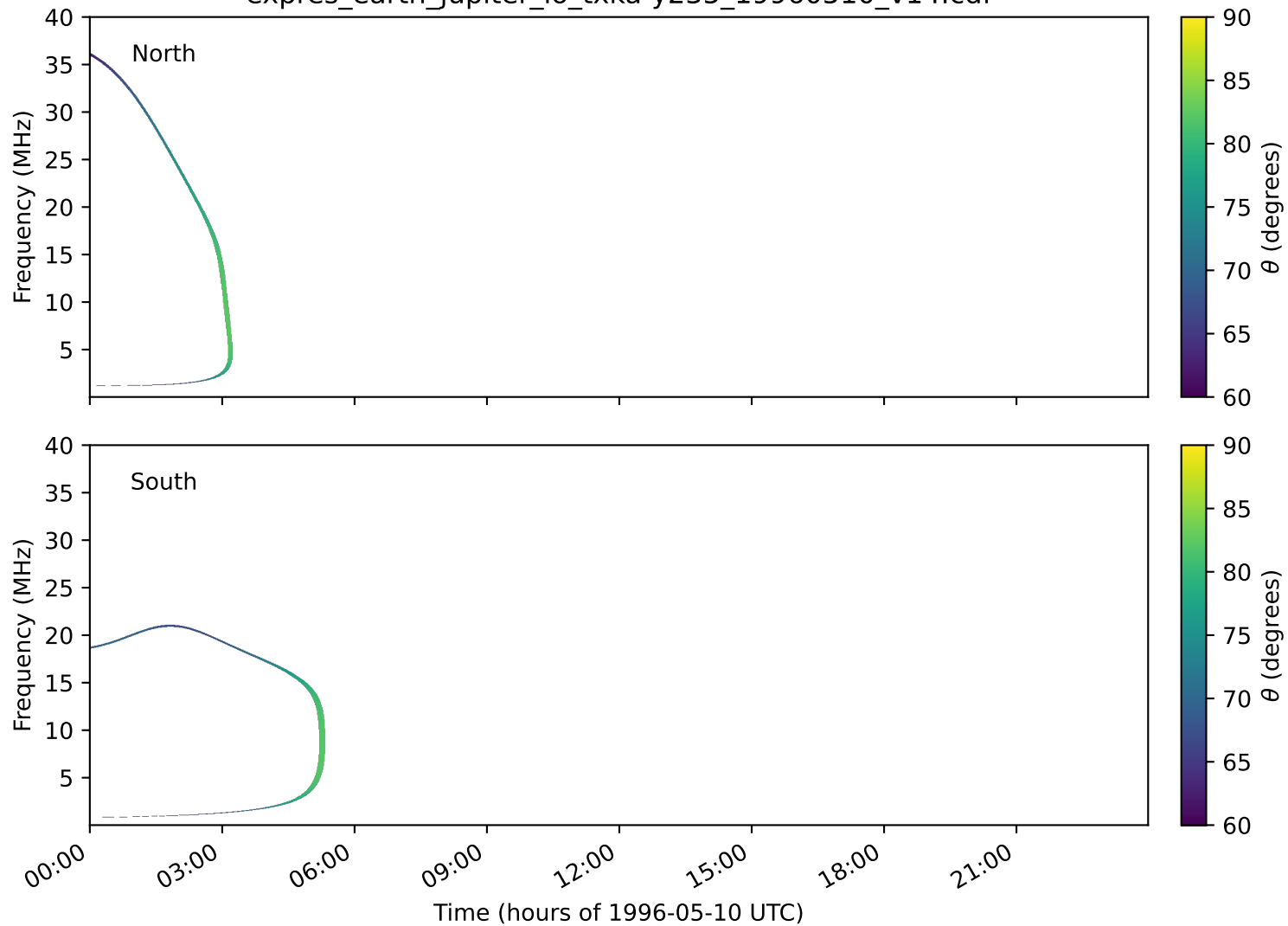
expres_earth_jupiter_io_txka-y235_19960510_v14.cdf
