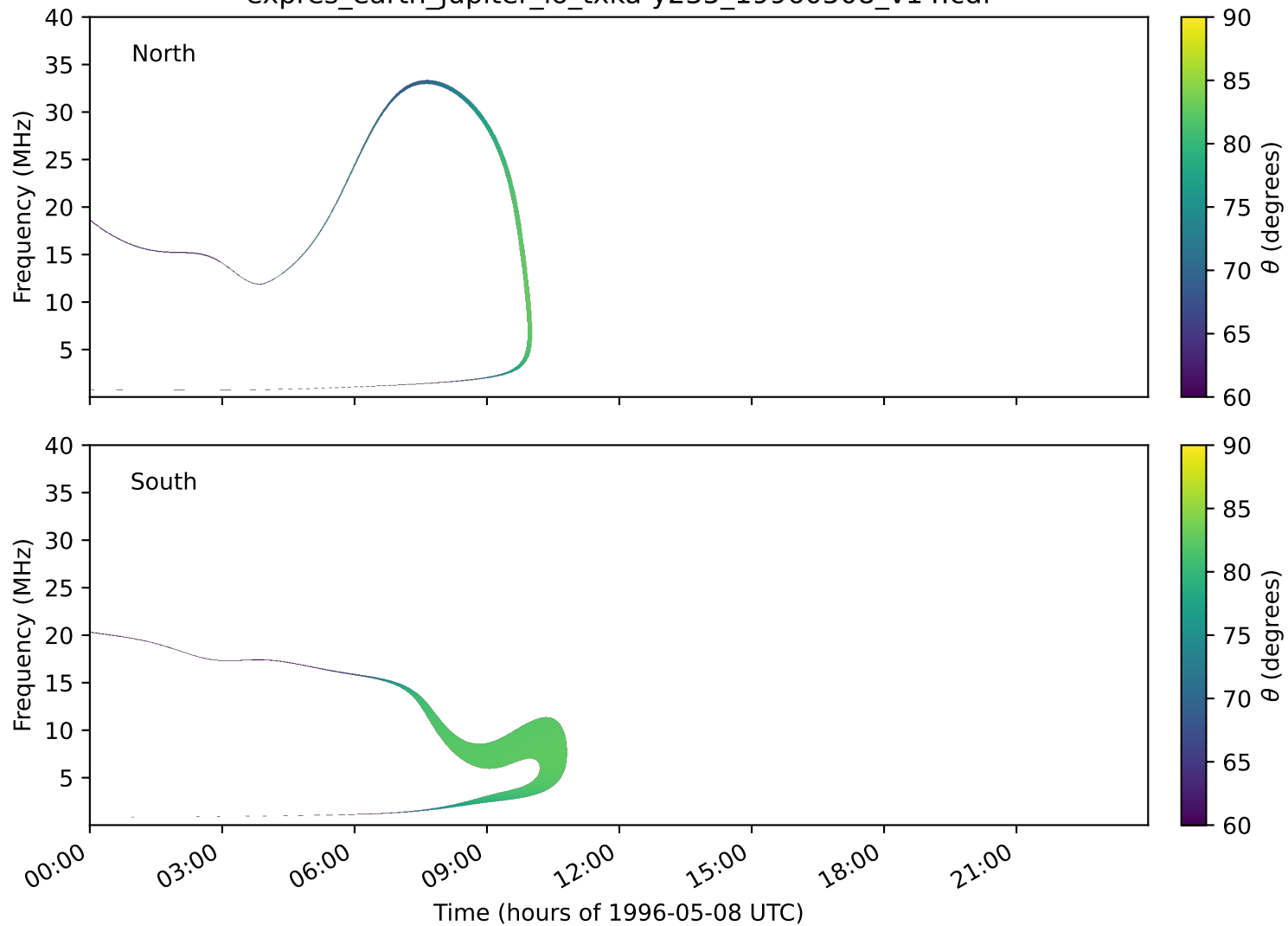
expres_earth_jupiter_io_txka-y235_19960508_v14.cdf
