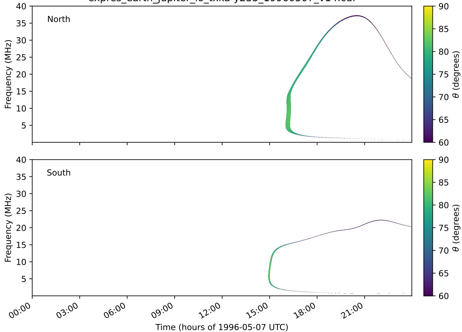
expres_earth_jupiter_io_txka-y235_19960507_v14.cdf
